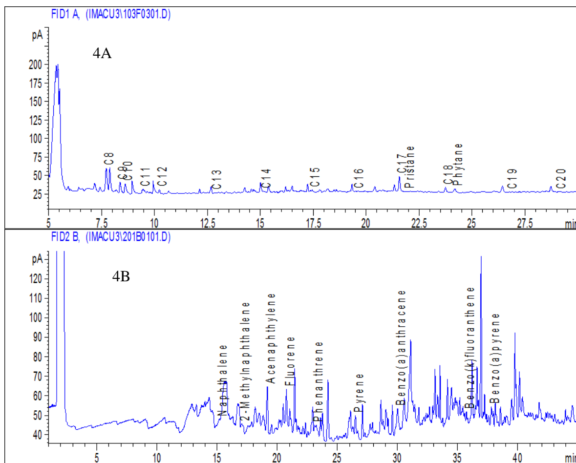
Figure 4: Chromatograms obtained from GC-FID analysis for aliphatic (A) and aromatic (B) hydrocarbon contents of 0% crude oil soil samples before planting
