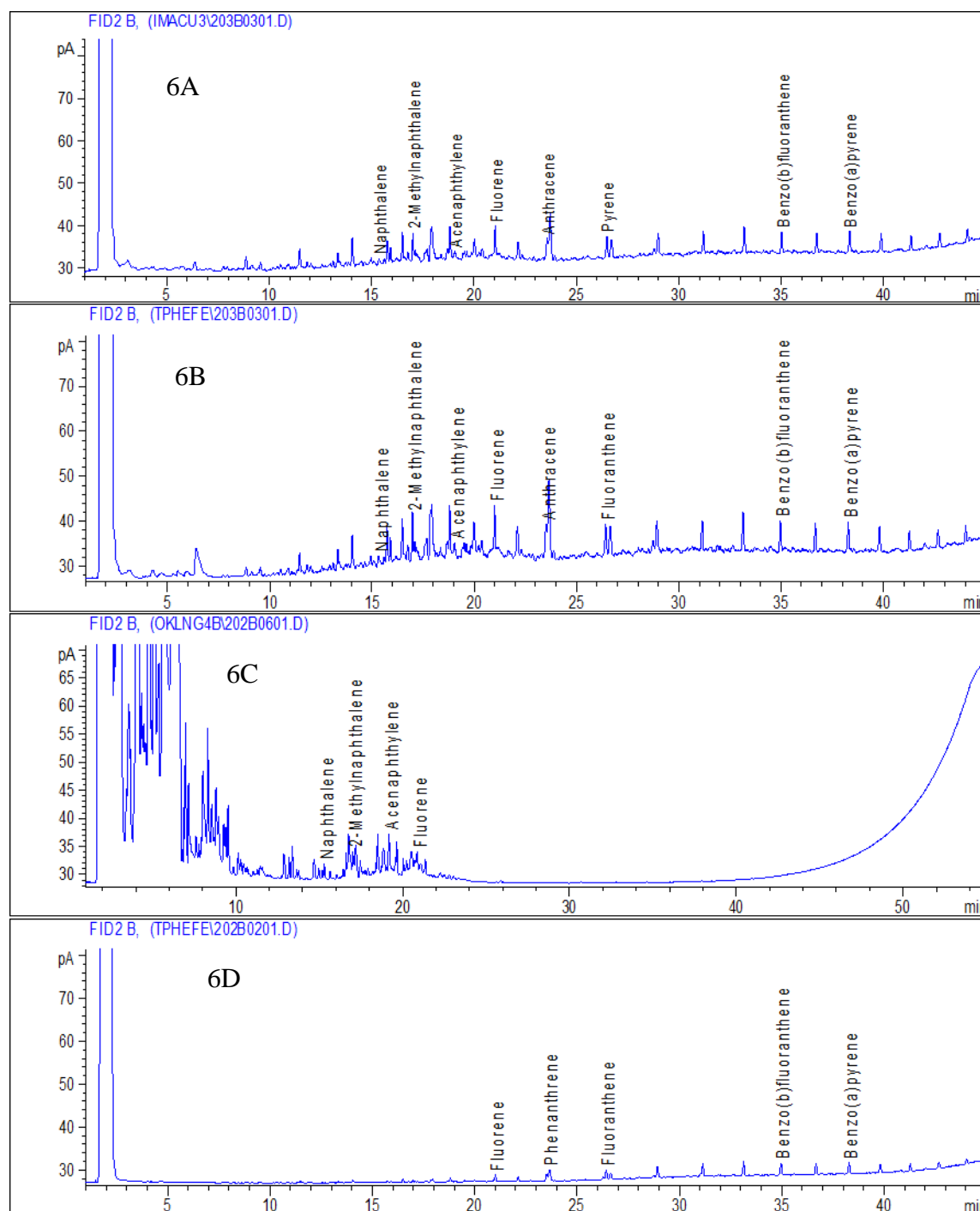
Figure 6: Chromatograms obtained from GC-FID analysis for aromatic hydrocarbon contents of 0% crude oil soil samples before planting (6A), 20% oil polluted soils after A. compressus (6B), C. dactylon (6C) and E. indica (6D) growth for 120 days.
