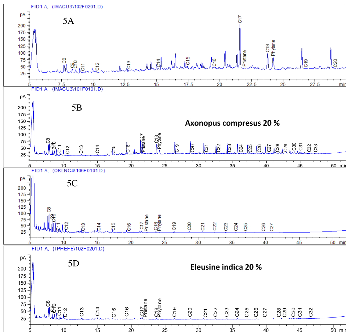
Figure 5: Chromatograms obtained from GC-FID analysis for aliphatic hydrocarbon contents of 20% crude oil soil samples before planting (5A), 20% oil polluted soils after A. compressus (5B), C. dactylon (5C) and E. indica (5D) growth for 120 days
