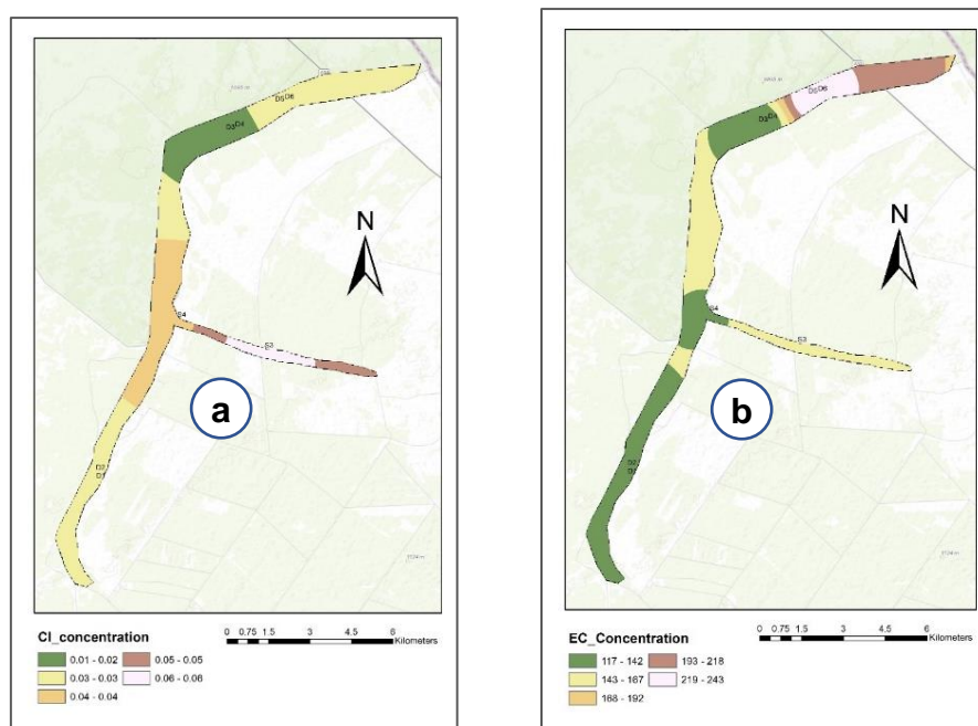
Figure 4: Spatial Distribution of Cl - (a), EC (b), HCO 3 - (c), Na + (d), SAR (e) and IWQI (f) for ADW Within the Main Drainage Channel in the Study Area
